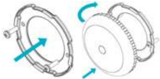
Figure 17: Installing Sensor on Ceiling
