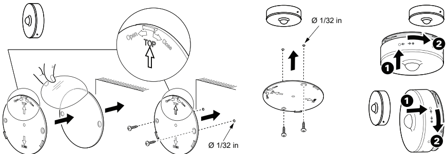
Figure 38: Ceiling/Wall Sensor Installation
