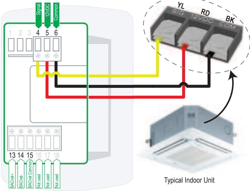
Figure 5: Controller Wiring
