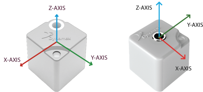
Figure: Axes orientation Left: DynaLogger TcA+. Right: DynaLoggers HF and HF+
