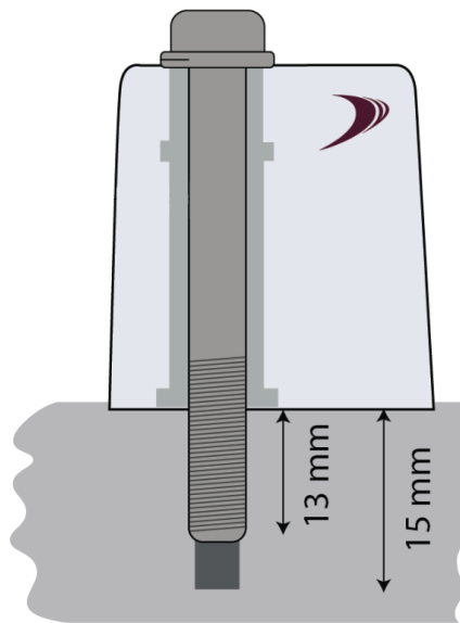
Figure: Screw Mounting
