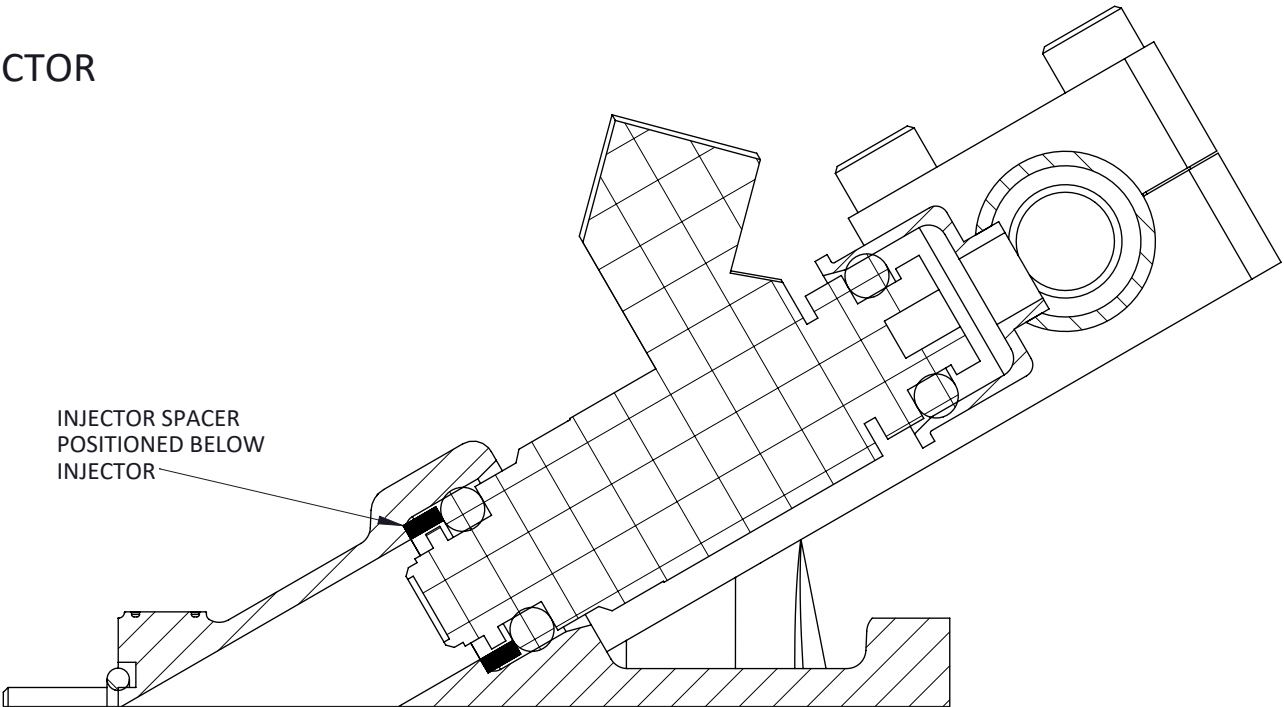
SECTION VIEW OF INJECTOR IN SF BODY
