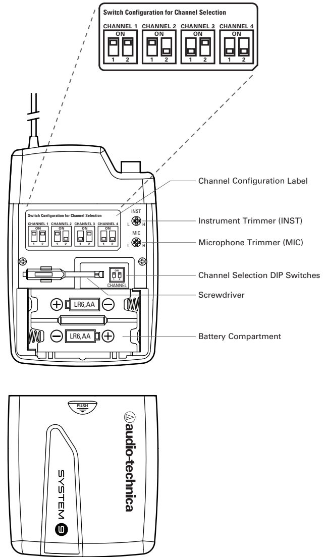
Figure D — UniPak® Transmitter
