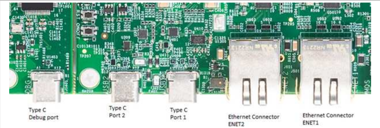
Figure 45. i.MX 93 port layout
