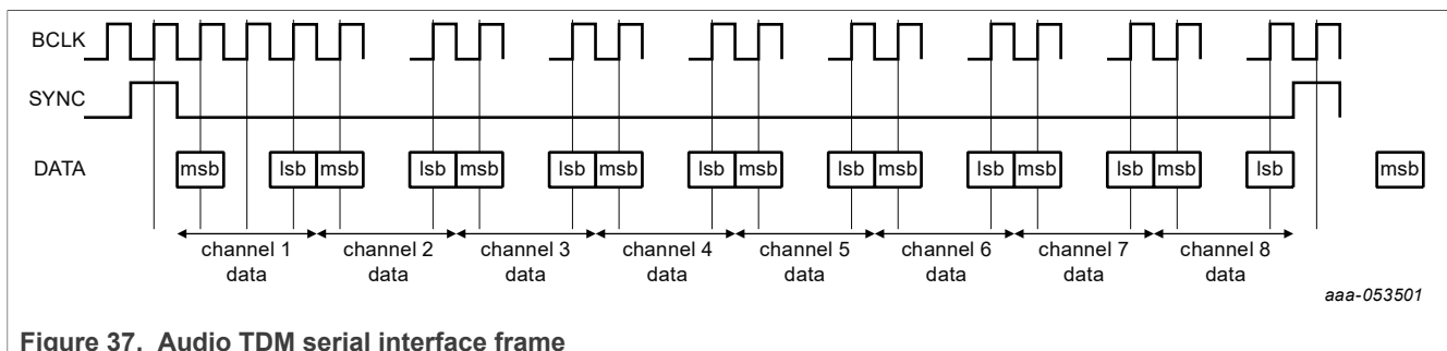
Figure 37. Audio TDM serial interface frame
