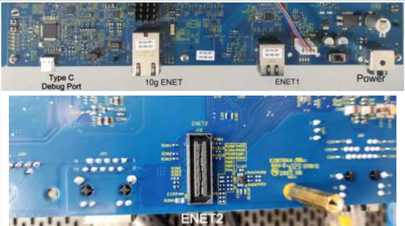
Figure 46. i.MX 95 port layout
