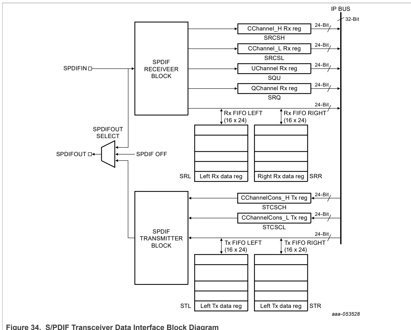
Figure 34. S/PDIF Transceiver Data Interface Block Diagram
