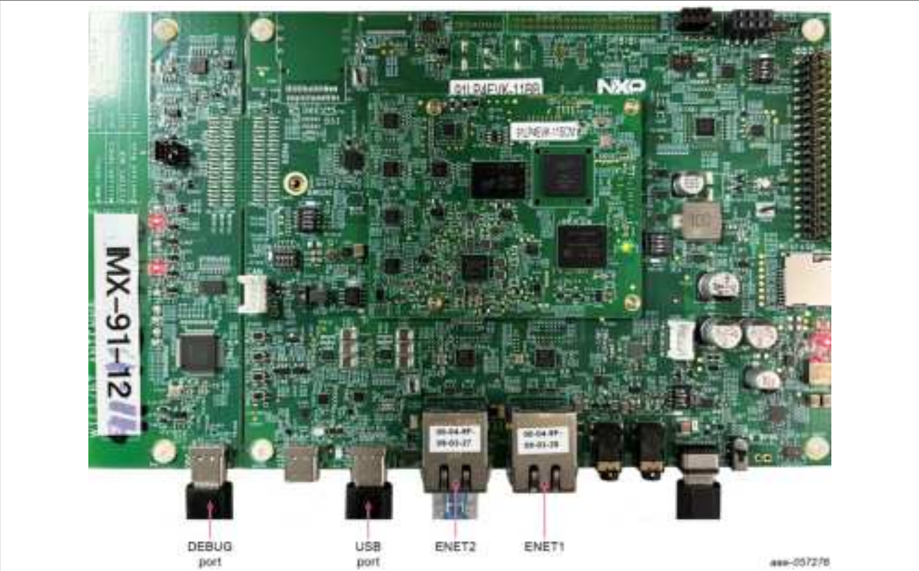
Figure 44. i.MX 91 EVK Port Layout
