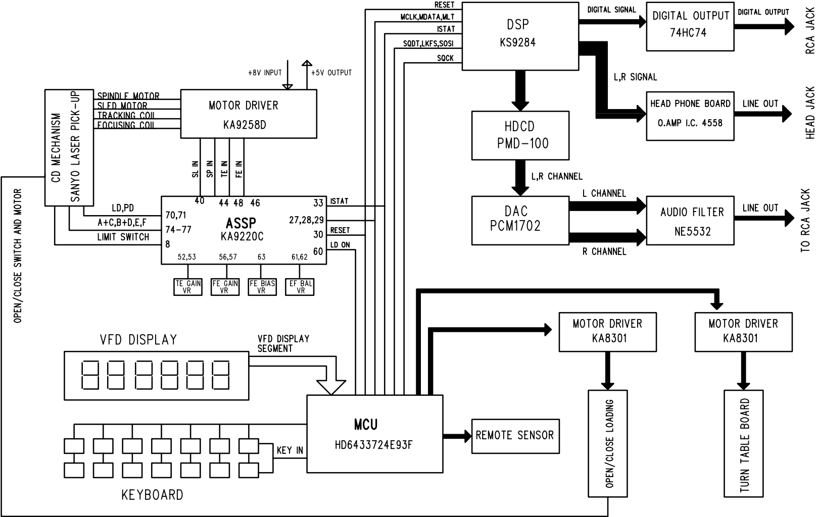
FL8550 BLOCK DIAGRAM OF SAMSUNG CHIPSET I
