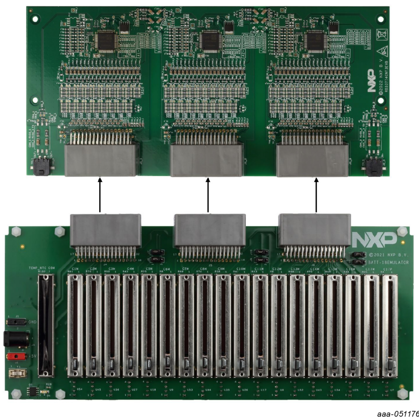
Figure 8. Battery emulator connection
