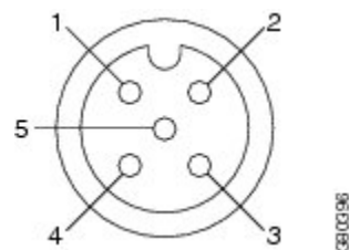
Figure 6: Console Connector
