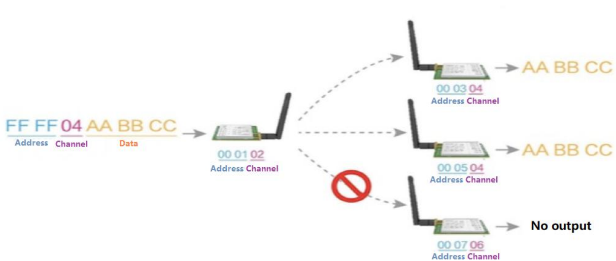
Figure 5-2 Broadcasting Transmission
