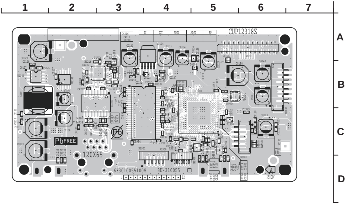
ETHERNET PCB (COMPONENT SIDE)
