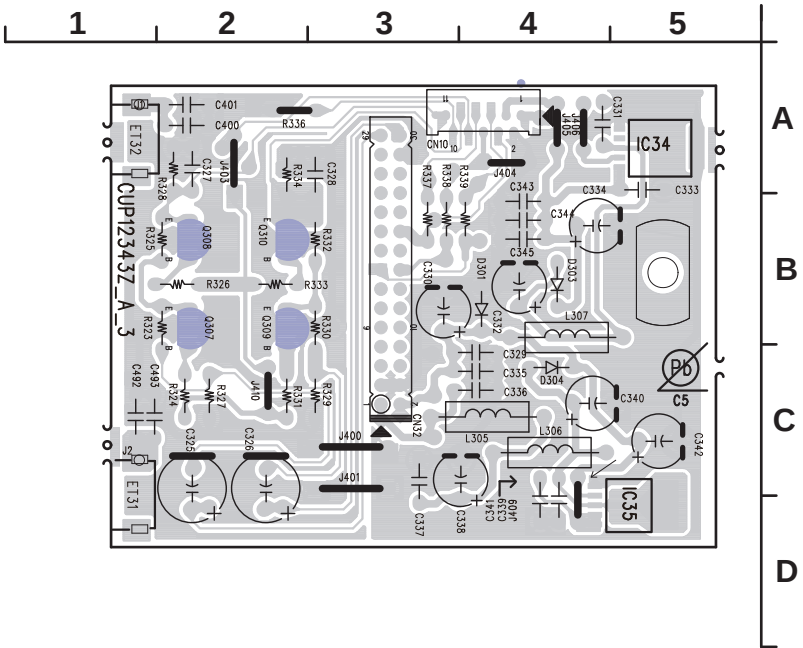
DAB PCB (COMPONENT SIDE)
