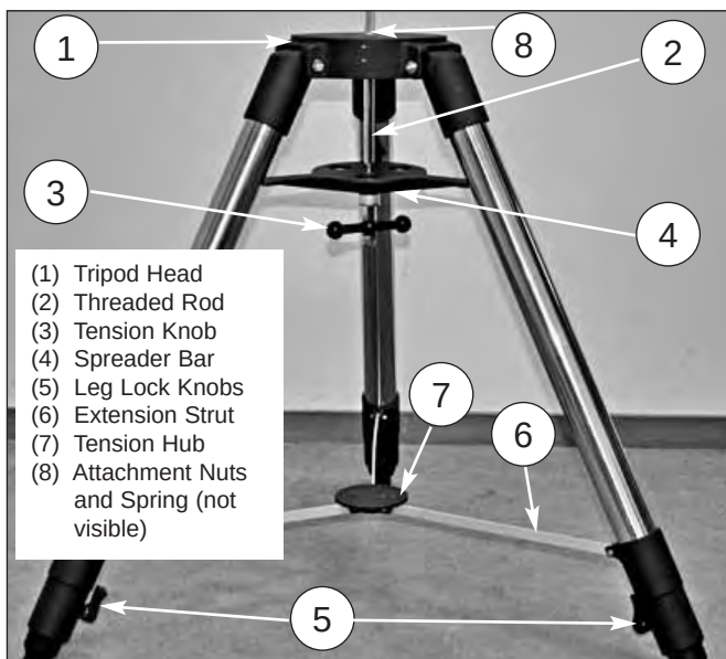
Fig. A: Field Tripod with legs extended.
