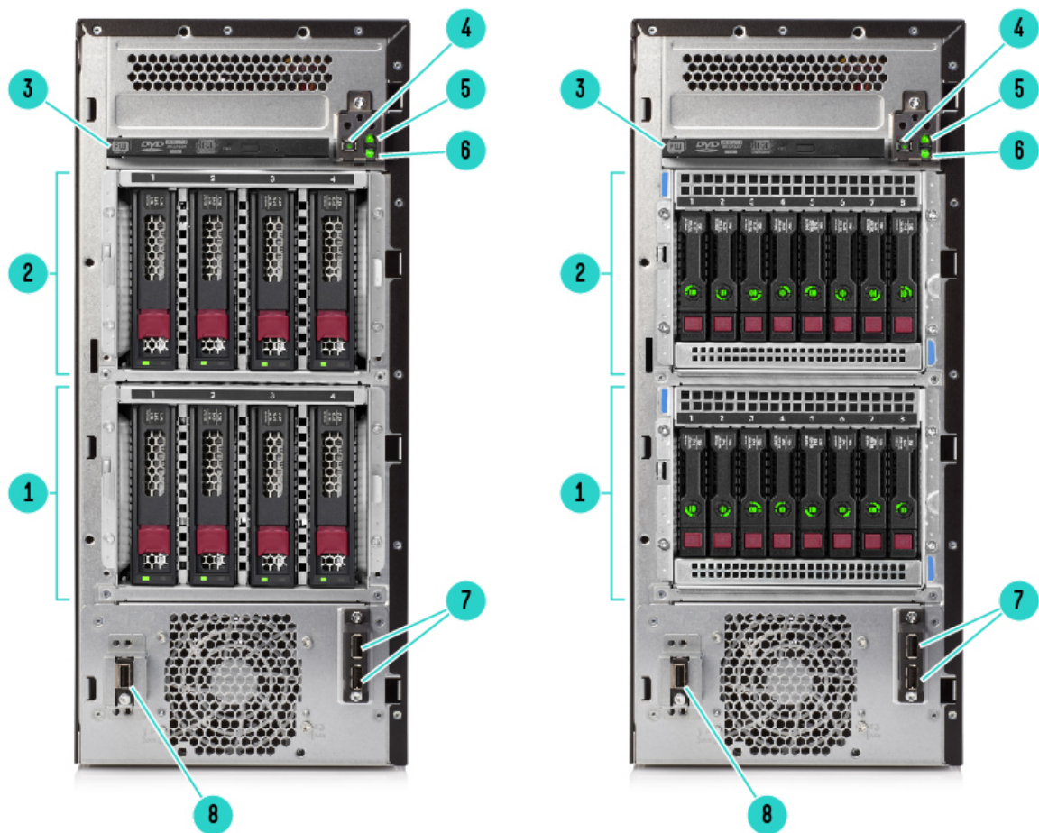
Front View (details for 8LFF and 16SFF)
