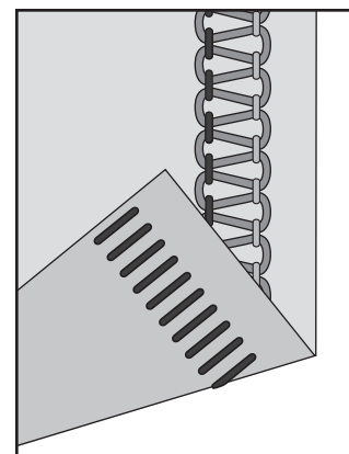
3-thread flatlock stitch
