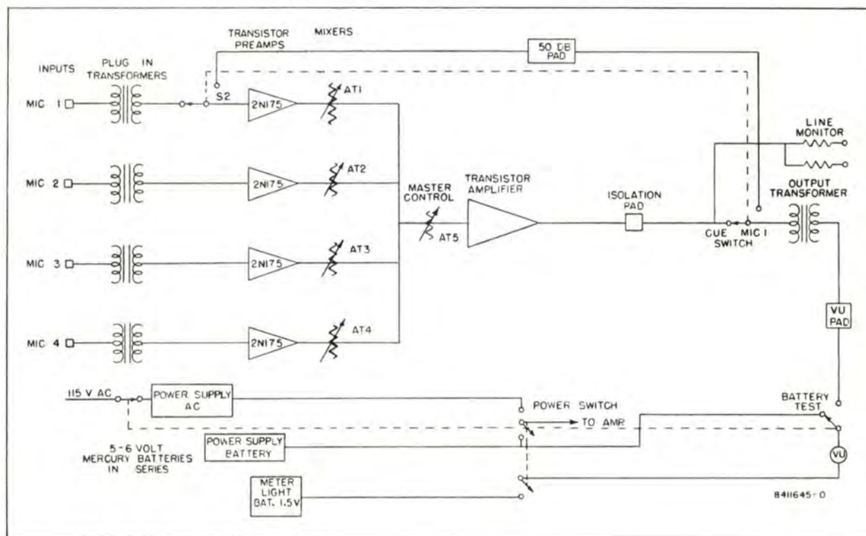
Figure 3 - Block Diagram
