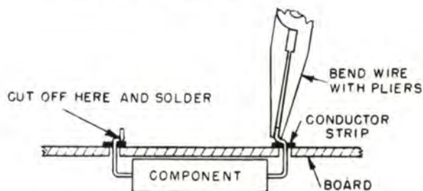
TO REMOVE COMPONENT FROM TOP OF CIRCUIT BOARD
