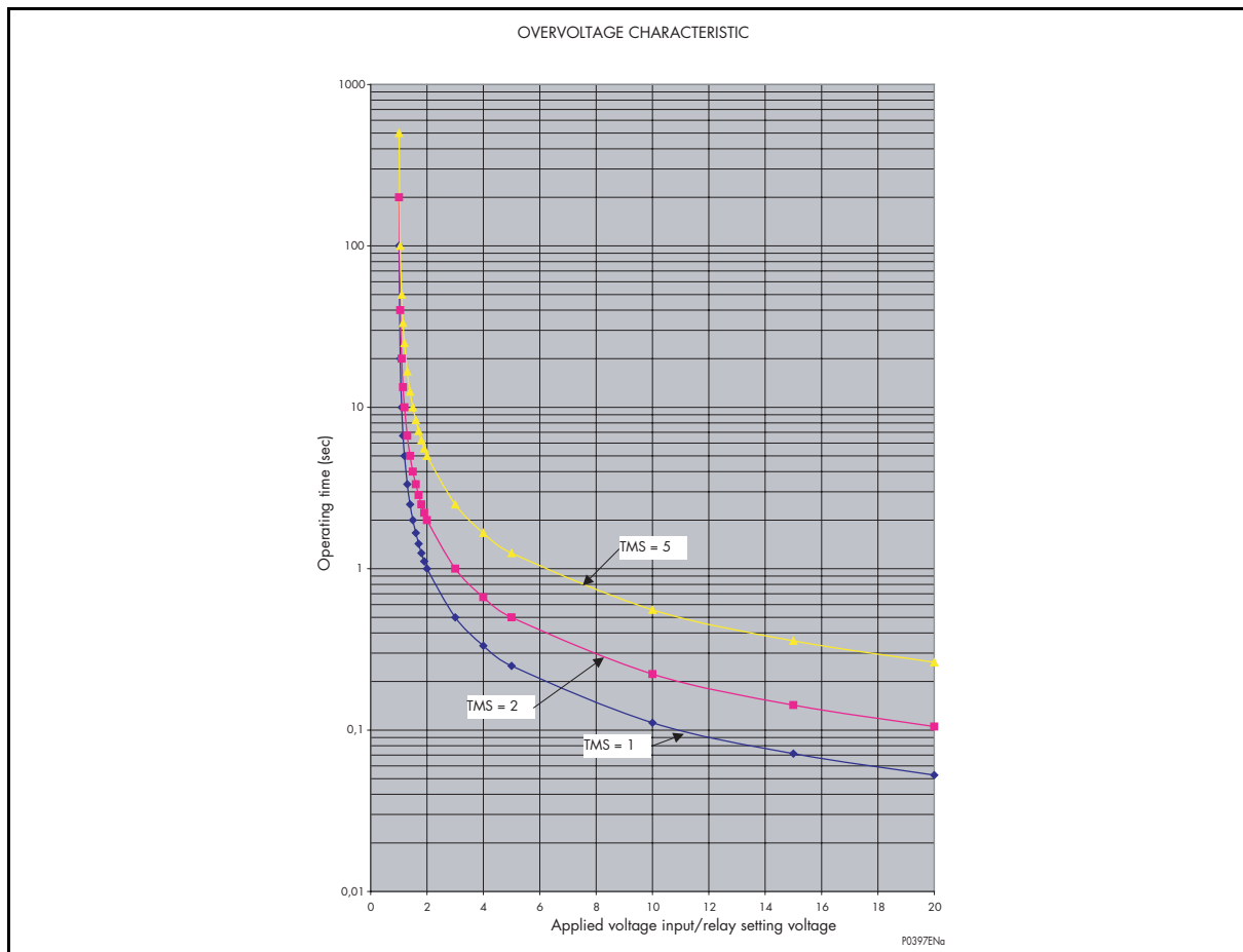
IDMT CURVE FOR THE OVERVOLTAGE ELEMENT "V&gt;"
