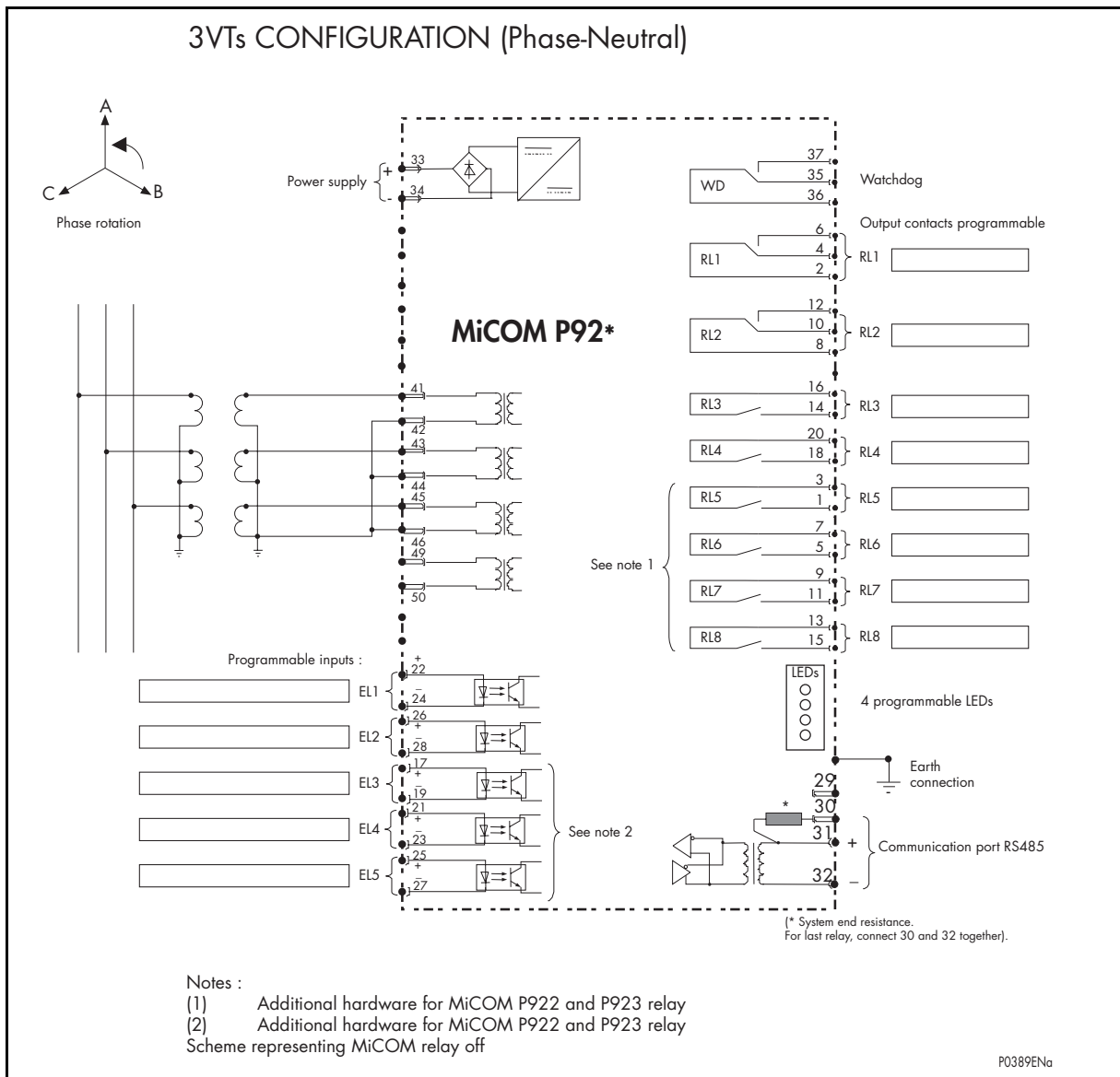
FIGURE 1: 3VTs CONNECTION
