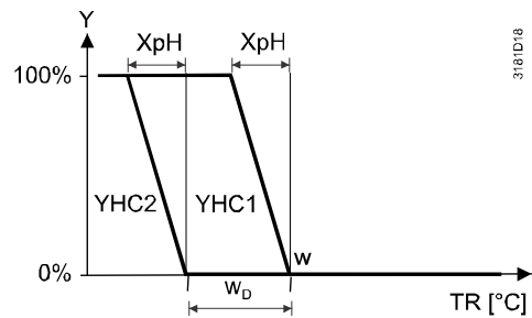
Heating mode (P01=0)
