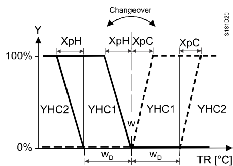
Changeover (P01=2 or P01= 3)
