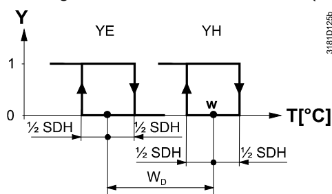
Heating mode with manual selection (P01=2)
