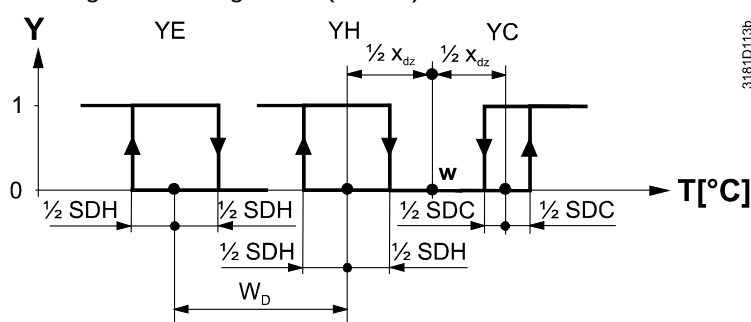
Heating and cooling mode (P01=4)
