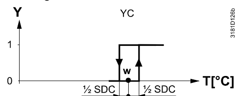
Cooling mode with manual selection P01=2
