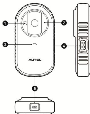
Figure 2-4 XP200 Views
