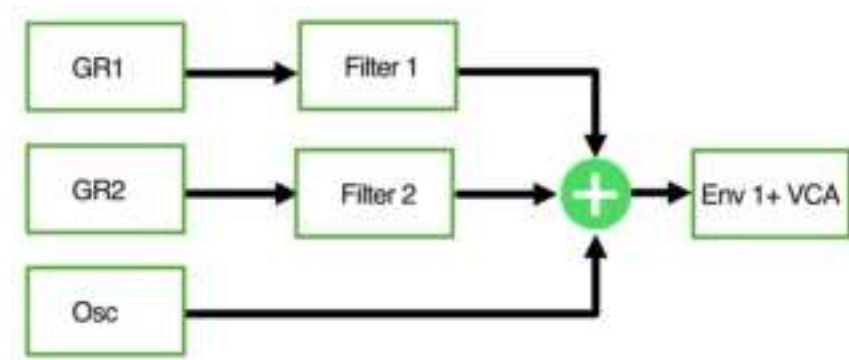
Figure: Granular Track Voice Signal Flow with Per-Oscillator Filter Configuration
