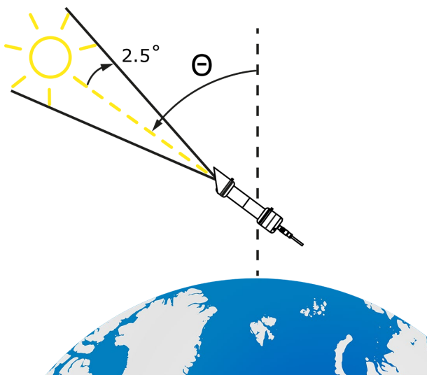
Figure 4 Pyrheliometers measure only the sunlight from a small area around the sun, characterised by a opening half-angle of 2.5^\circ .
