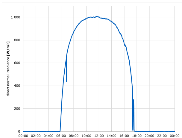
Figure 3 Direct normal irradiance as measured by a DR30 pyrheliometer. Data taken 25 September 2019, during the NREL National Pyrheliometer Comparison.
