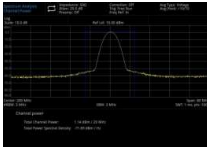
Figure 5-1 Channel Power
