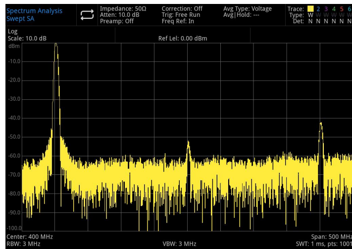
Figure 3-16 Harmonic Distortion
