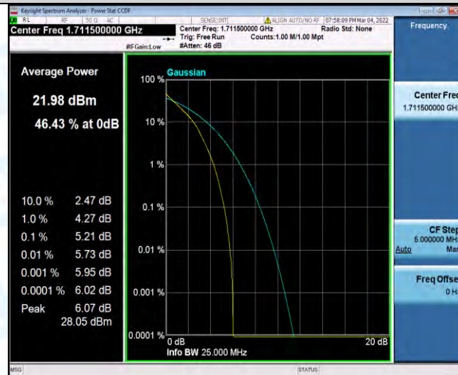
Band4-3MHz-QPSK-20175-1RB#0
