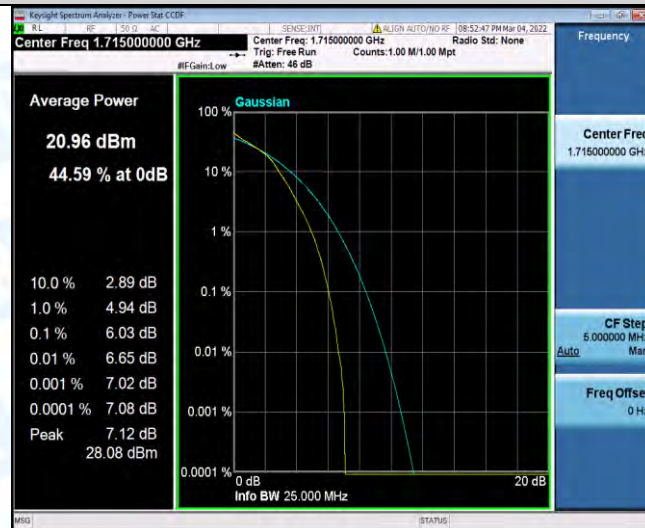
Band4-10MHz-16QAM-20175-1RB#0
