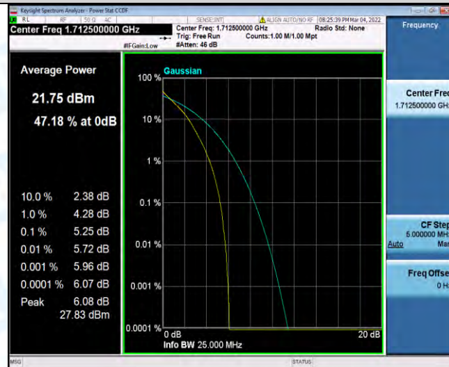
Band4-5MHz-QPSK-20175-1RB#0
