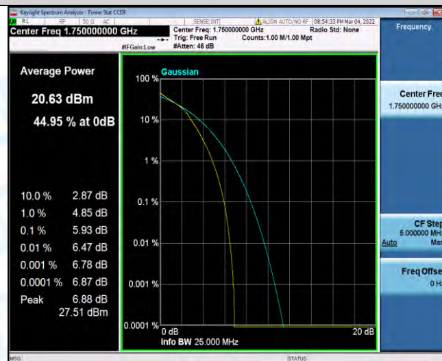
Band4-15MHz-QPSK-20025-1RB#0
