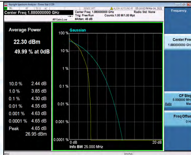
Band2-3MHz-QPSK-18900-15RB#0
