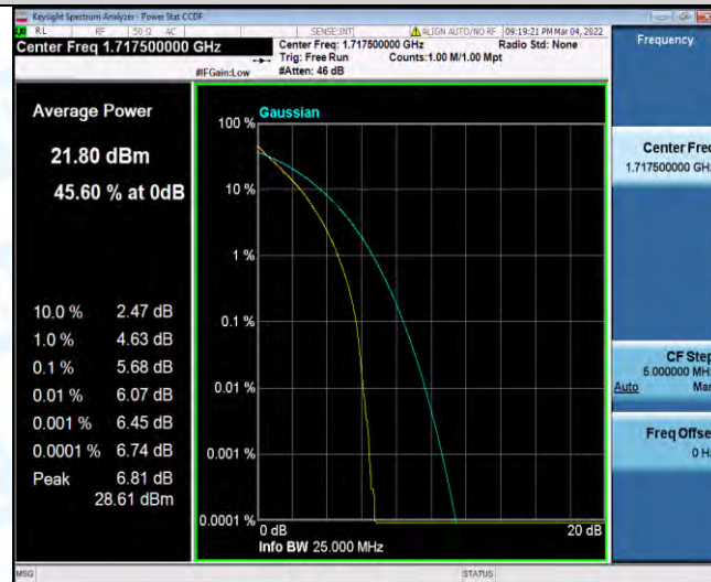
Band4-15MHz-QPSK-20175-1RB#0
