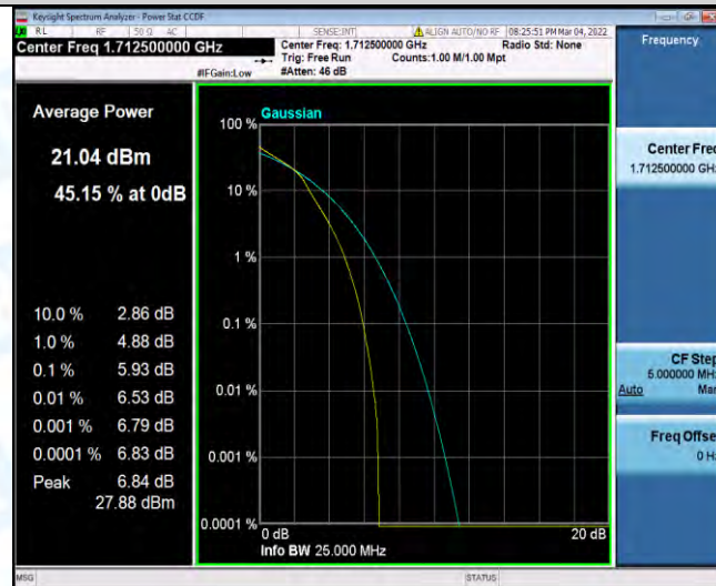
Band4-5MHz-16QAM-20175-1RB#0
