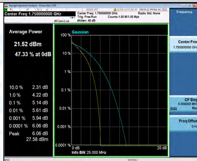
Band4-10MHz-16QAM-20000-1RB#0
