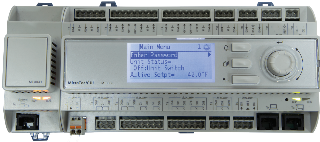
Figure 3: BACnet IP Communication Module Attached to Unit Controller (MicroTech III controller shown)
