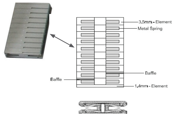
Figure 5: Board-to-Board Connector
