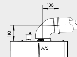
Concentric kit dimensions Ø 80/125
