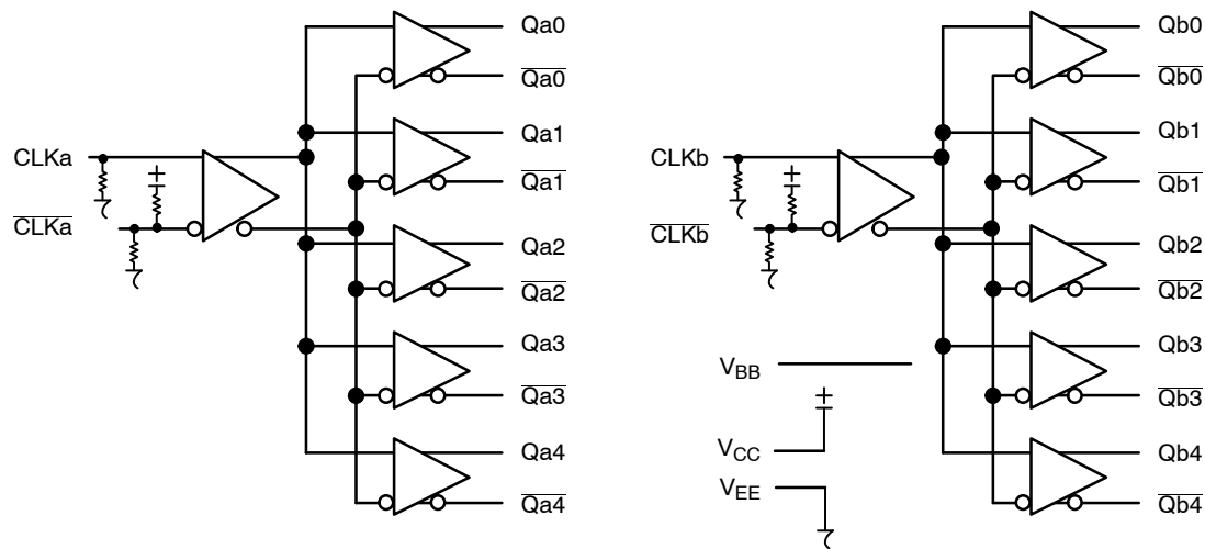
Figure 2. Logic Diagram
