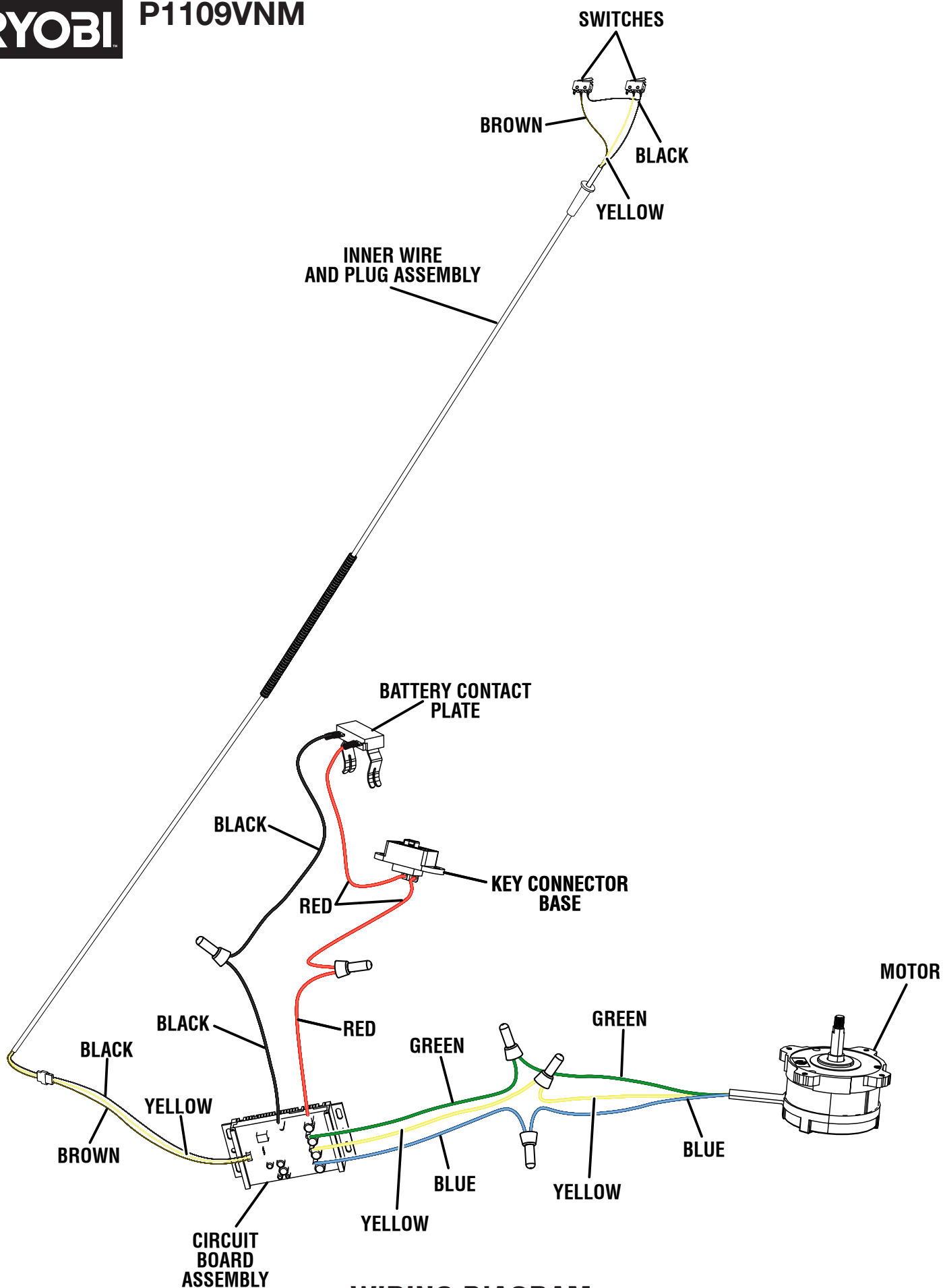
WIRING DIAGRAM
