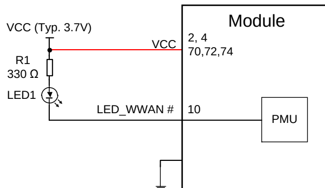
Figure 22: LED_WWAN# Reference Circuit
