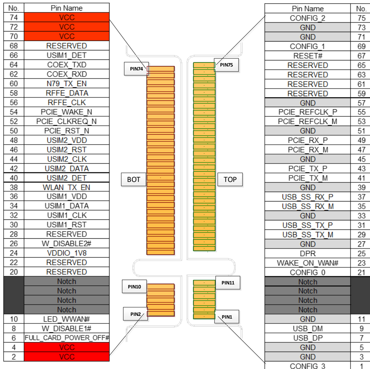
Figure 2: Pin Assignment
