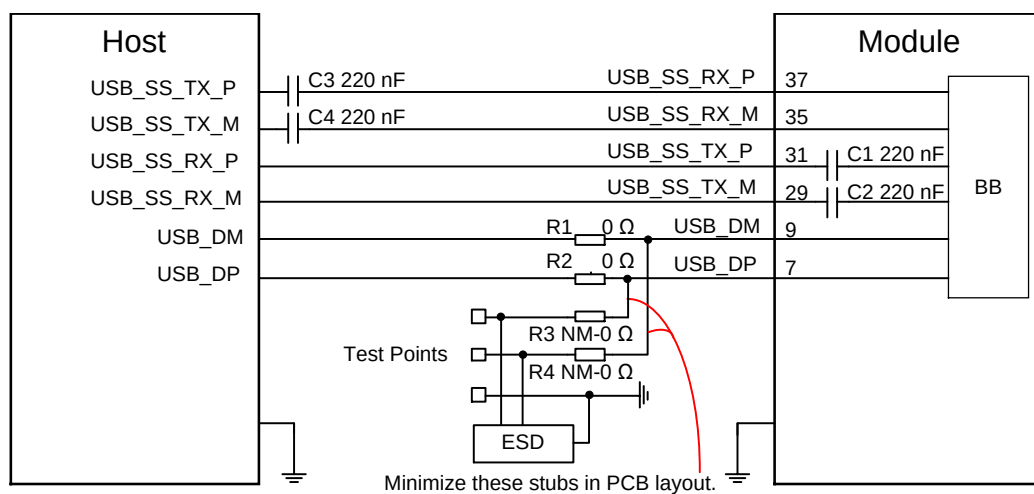
Figure 19: Reference Circuit of USB 3.1 & 2.0 Interfaces
