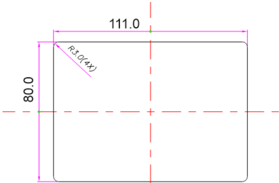
PANEL CUT OUT DIMENSIONS
