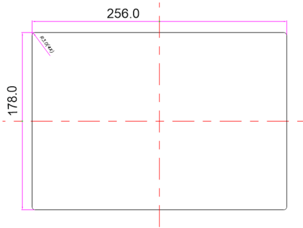
PANEL CUT OUT DIMENSIONS
