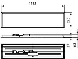
RC132V G5 PSU W30L120 OC
