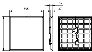
RC132V G5 PSU W60L60 OC
