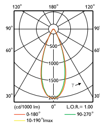
RS150_151B LED6 WB
