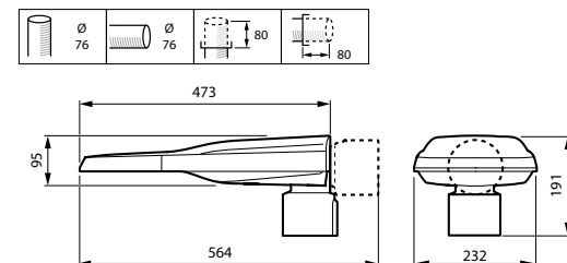
UNI LUMISTREET GEN2 MICRO 76
