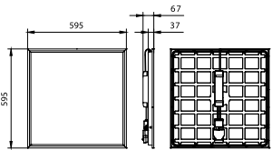
RC132V G5 PSD W60L60 OC
