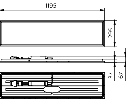
RC132V G5 PSD W30L120 OC
