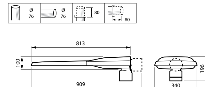
UNI LUMISTREET GEN2_LARGE 76
