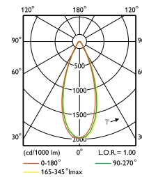
RS150_151B LED9 WB
