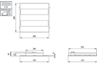
RC340B CPC_PCV W60L60
