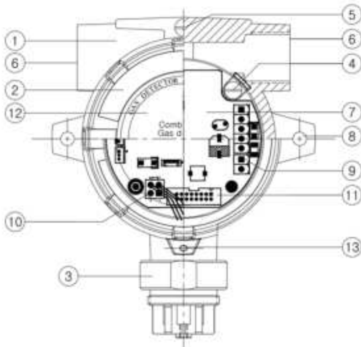
Figure 2. Tox Point 2000 Components
