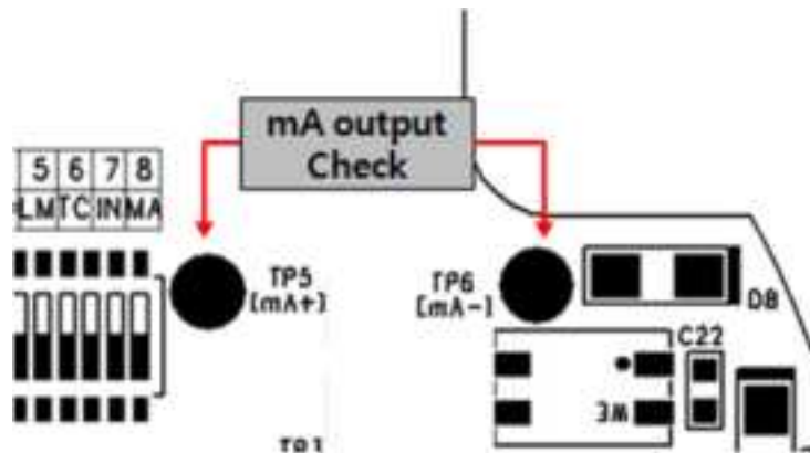
Figure 8. 4-20mA Output Test Terminal
