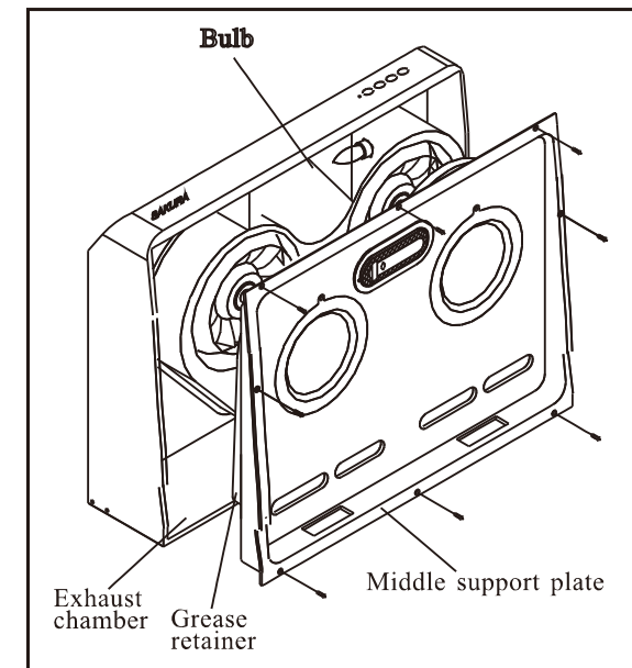
Fig. 10 Remove the middle support plate
