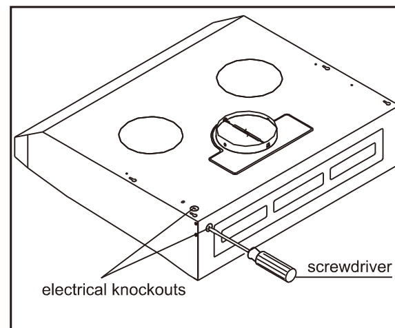
Fig.5 Electrical knockouts
