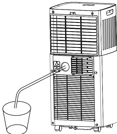
Continuous drainage (Dehumidification mode)
