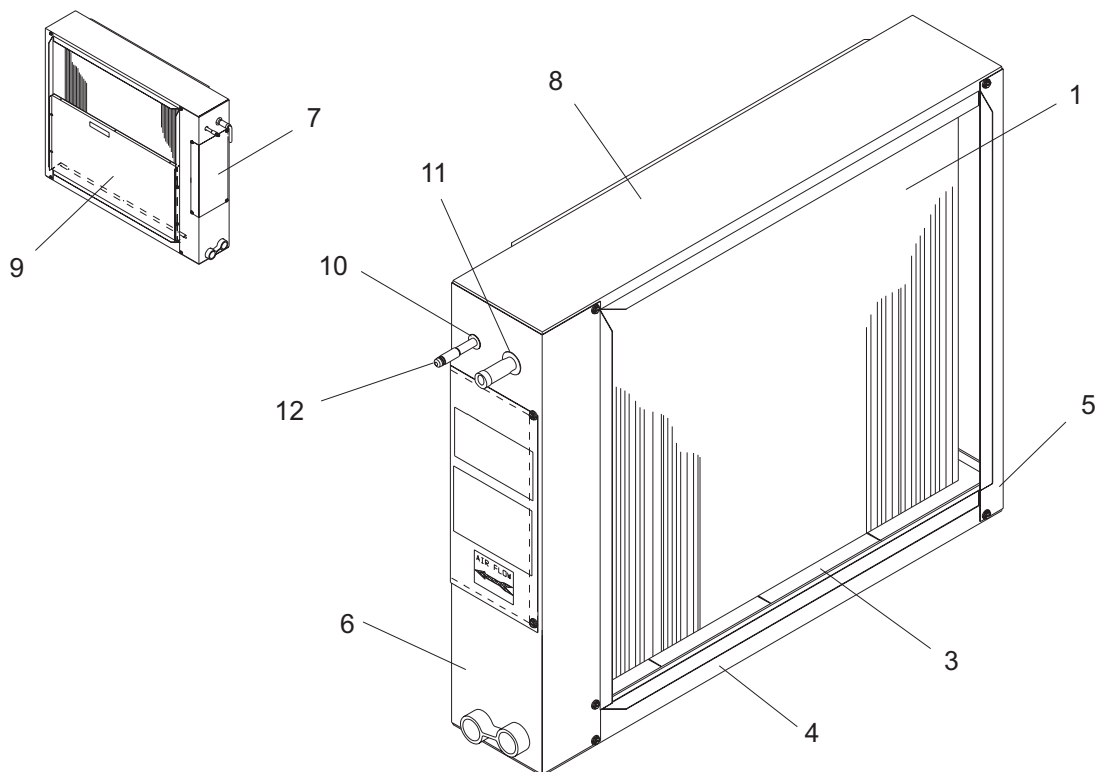
Figure 1 : HORIZONTAL DUCT COILS - R-22 TXV
