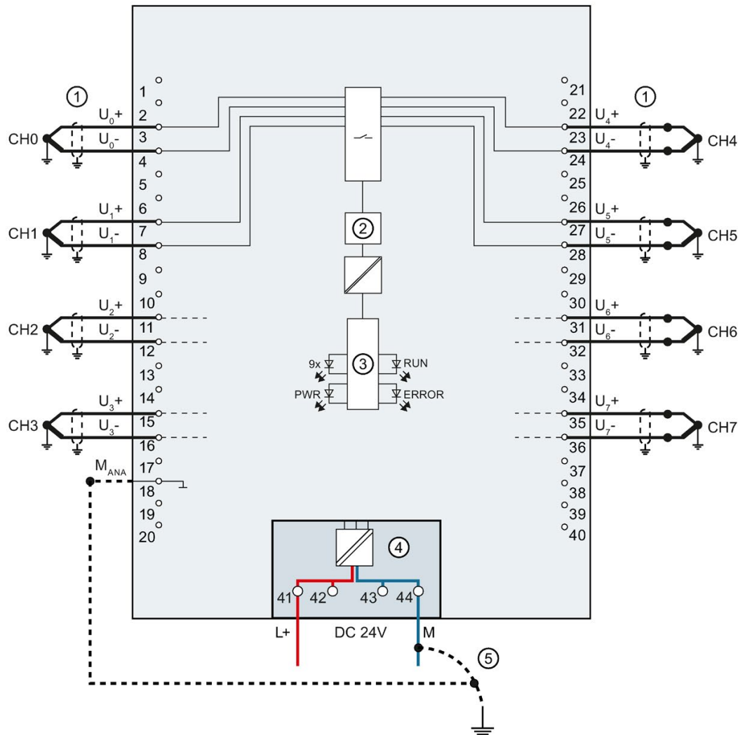
Figure 3-7 Block diagram and pin assignment for grounded thermocouples
