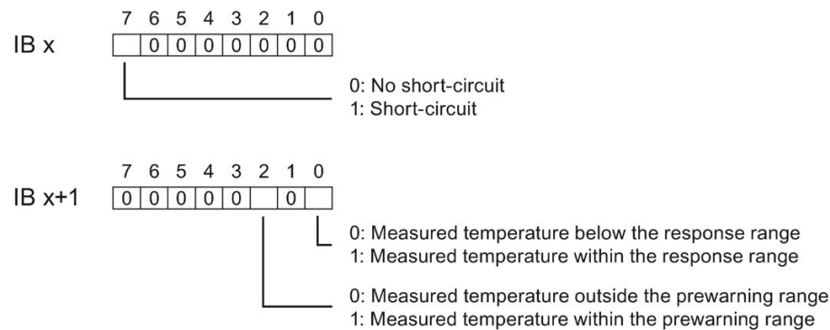
Figure 4-1 Address space for the AI 8xU/I/RTD/TC ST module with PTC resistors
