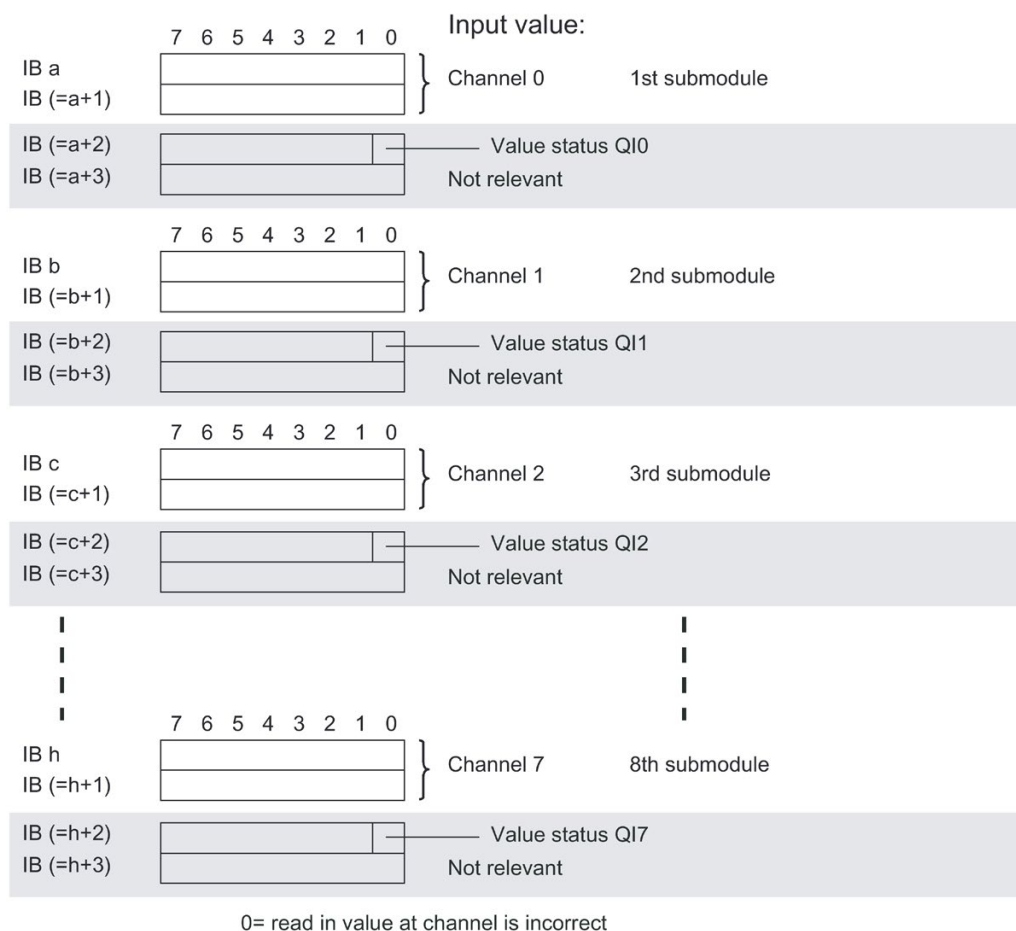
Figure 4-5 Address space for configuration as 8 x 1-channel AI 8xU/I/RTD/TC ST S QI with value status
