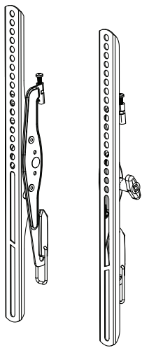
WALL PLATE
