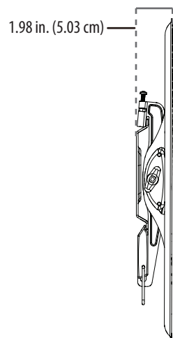
SIDE VIEW - RETRACTED
