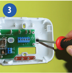
Fit the back of the receiver unit to the wall using the fittings supplied.
