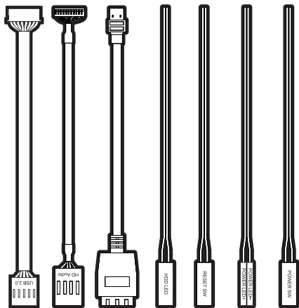
USB 2.0 HD Audio USB 3.0 HDD LED Reset SW Power LED Power
