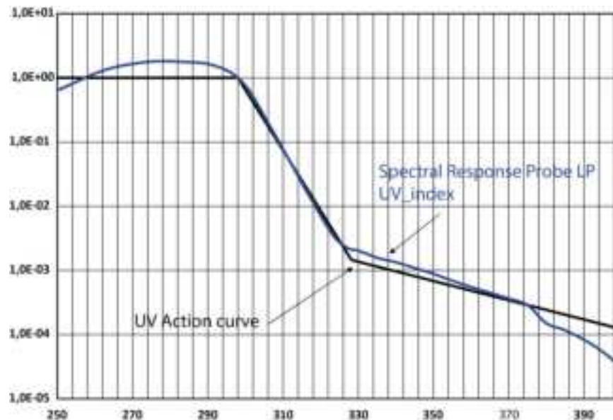
Fig. 3.1: spectral response
