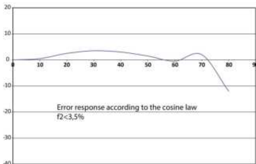
Fig. 3.2: directional error
