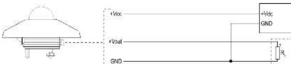
Fig. 4.4: LPUVI02...AV... connections
