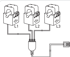
Current Transformer(1m) (x3)
