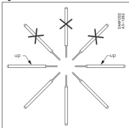
Figure 14: Sensor installation
