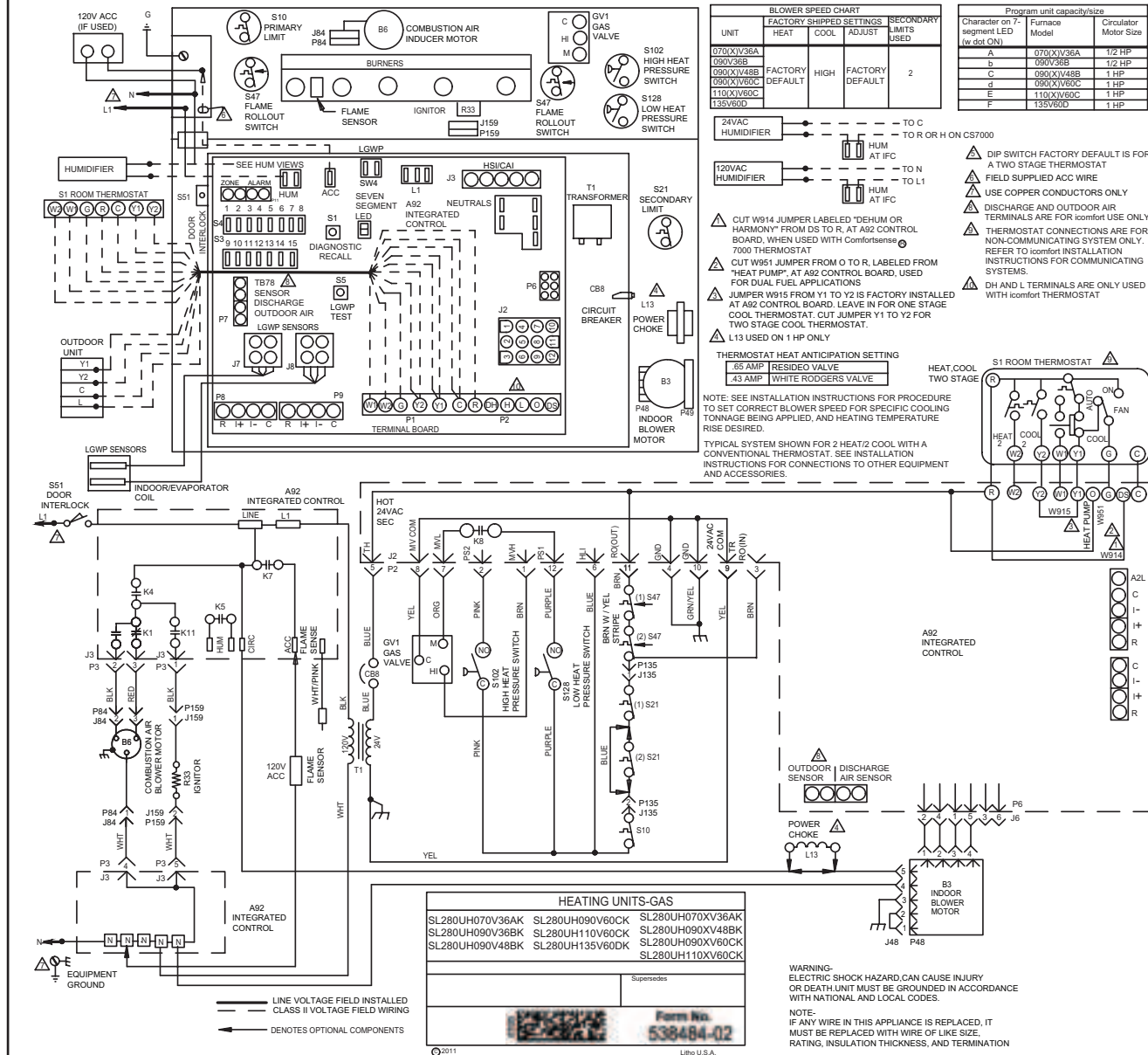
Wiring Diagram 538484-02
