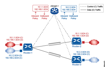
Figure 1: Propagation of Routing Information Inside a VRF
