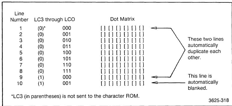
Figure 4-22. Display character format.
