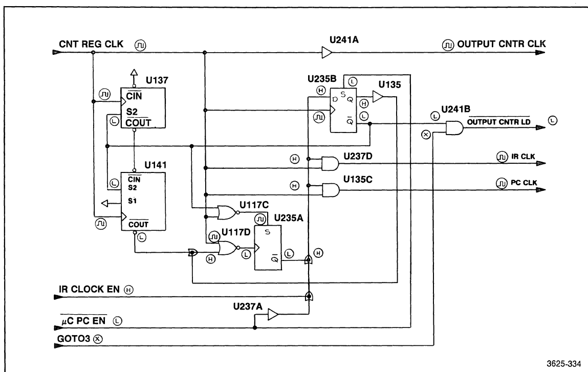
Figure 4-38. Clock control: non-count logic state.
