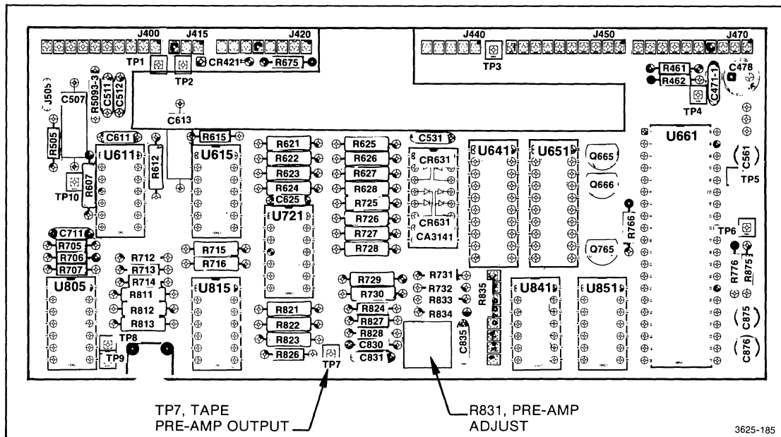
Figure 5-65. Tape Drive test point and adjustment locations.
