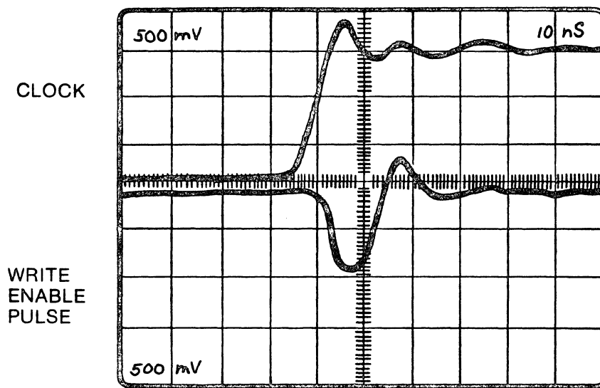
Figure 5-81. 91A08 write-enable timing.
