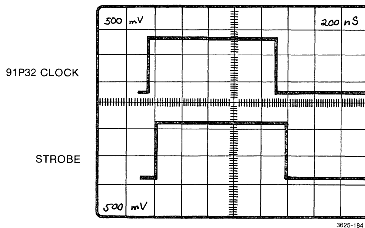
Figure 5-64. 91P32 strobe clock adjustment.
