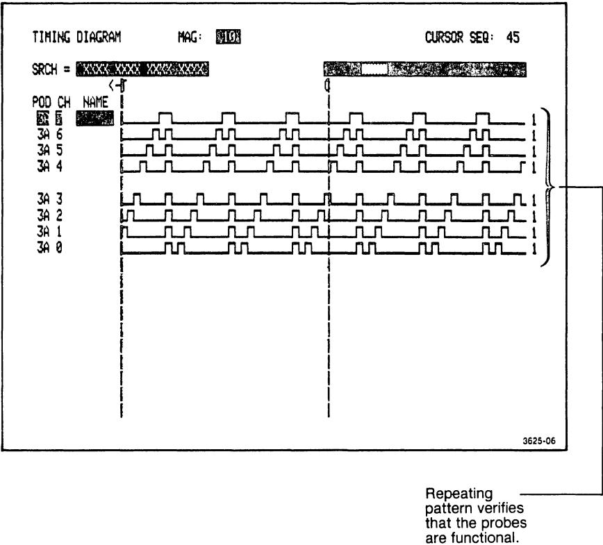
Figure 3-24 Timing Diagram display of probe self test.
