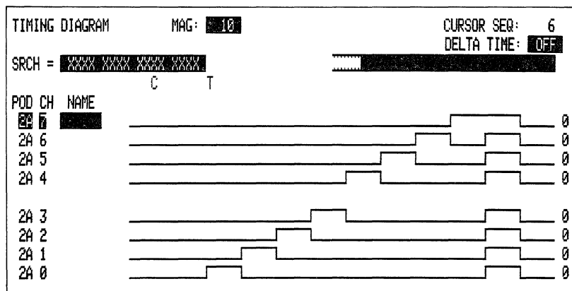
Figure 5-15. 5 \mu s pattern generator data acquired at 1 \mu s.
