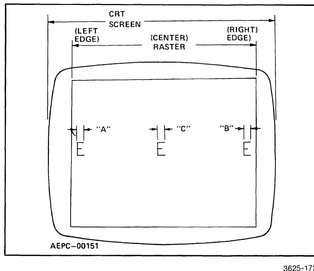
Figure 5-47. Linearity adjustment raster display.
