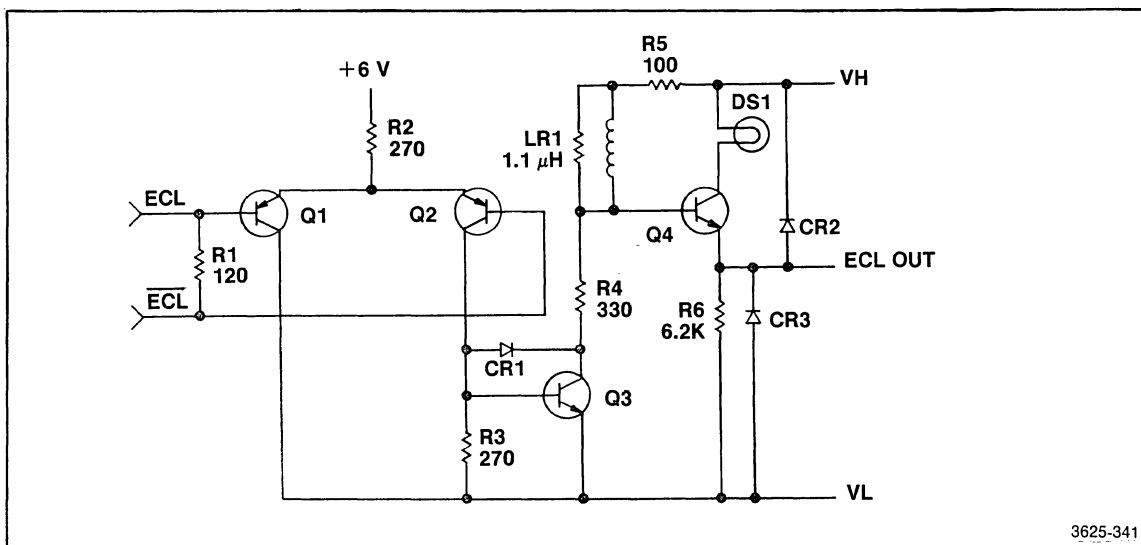
Figure 4-45. One channel of a P6456.
