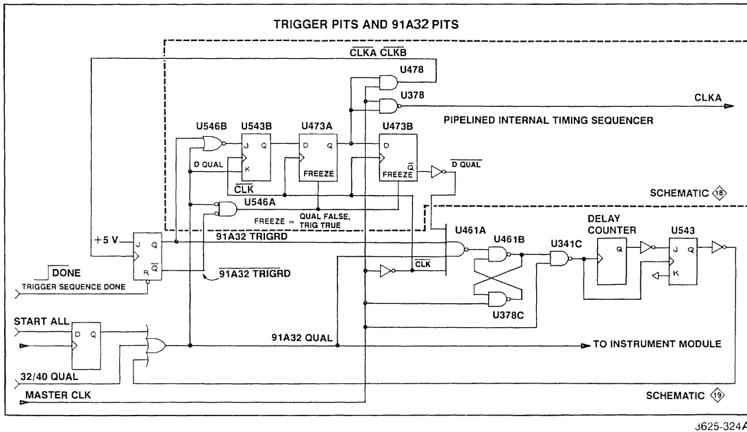
Figure 4-28. Simplified trigger shutdown circuit diagram.
