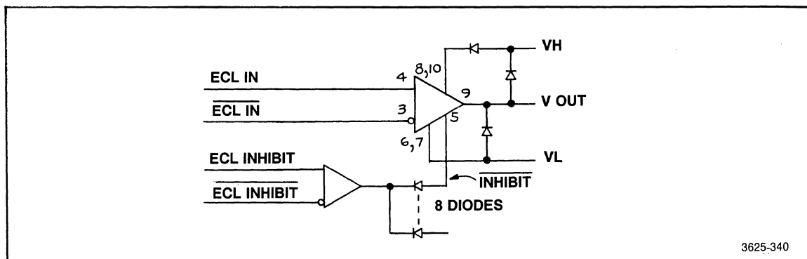
Figure 4-44. One channel of a P6455.
