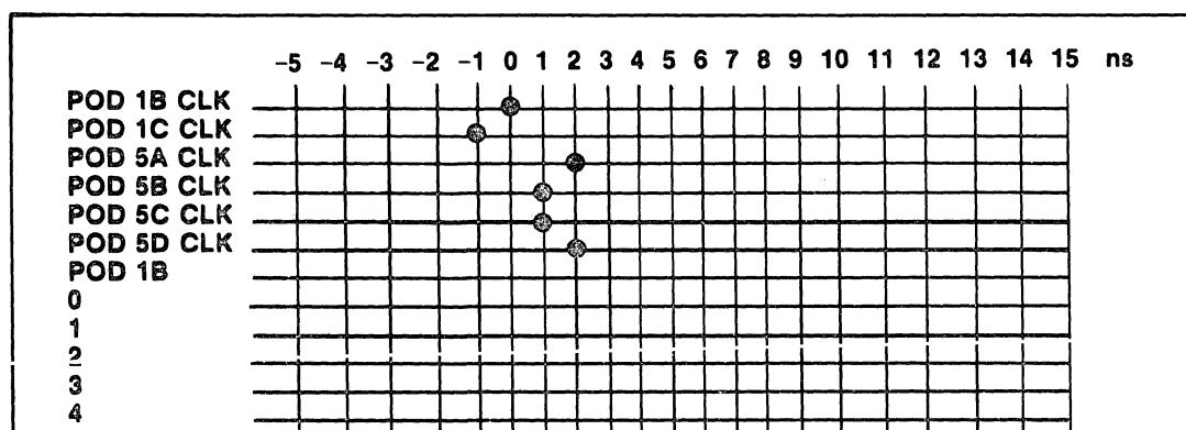
Figure 5-83. Example of clock skew data format.
