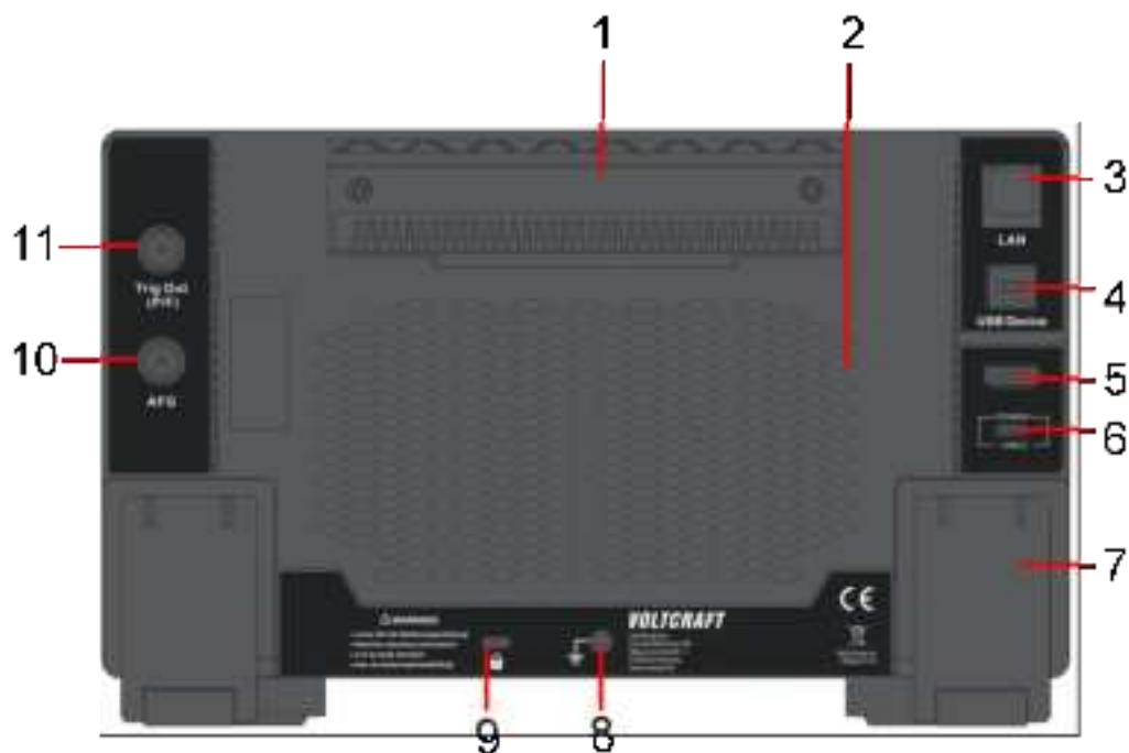
Figure 3-2: Rear Panel
