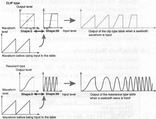
Shape of the wave shaping table and the Shape parameter
