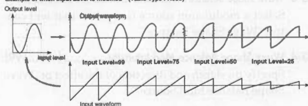
Example of when Input Level is modified (Table Type: Reso)
