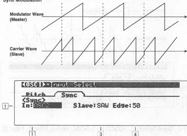
Sync Modulation
