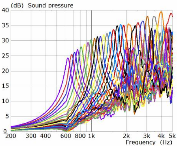
Figure 5. Pressure response at closed end of each absorption channel
