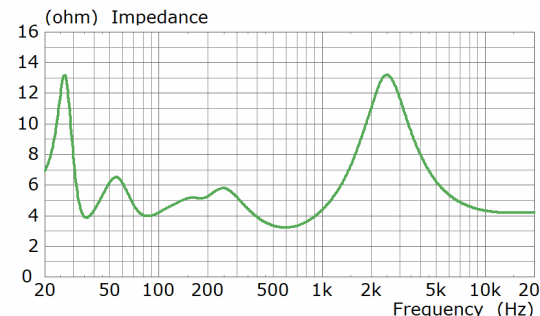
R11 Meta directivity contours - horizontal (top) and vertical (middle) - and impedance (bottom)
