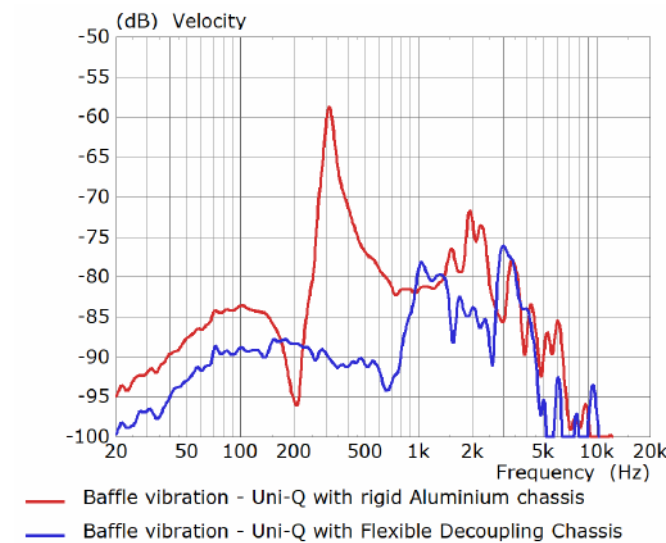
Figure 24. Effect of the Flexible Decoupling Chassis on baffle vibration
