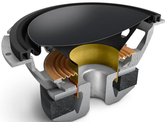
Figure 30. R Series LF driver
