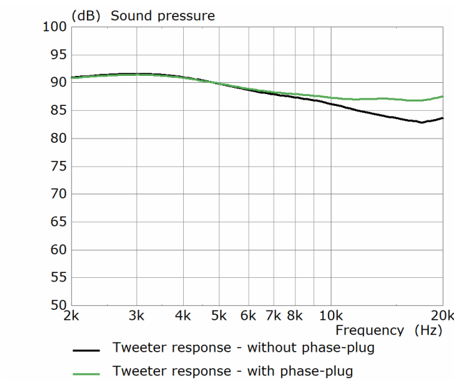
Figure 12. Effect of the Tangerine Waveguide compression chamber on the tweeter's axial response
