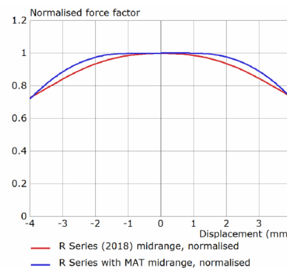
Figure 18. Midrange motor force factor BL(x) normalised to 0mm displacement
