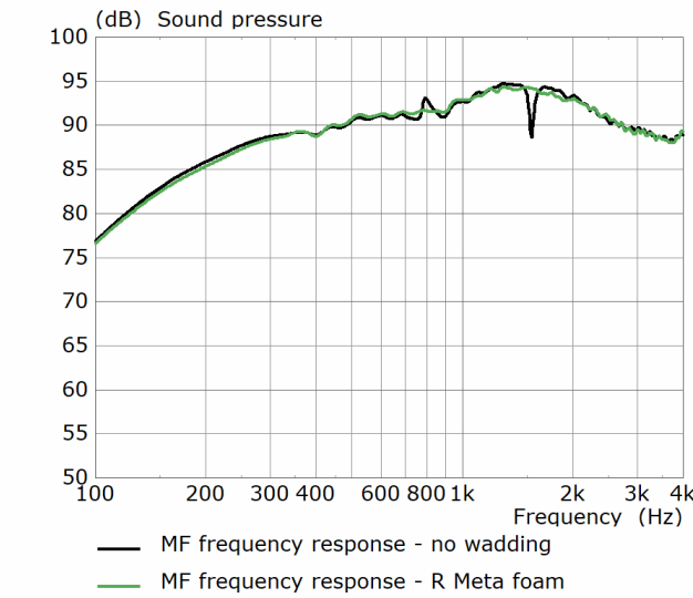
Figure 40. Measured frequency response of the midrange in R11 Meta (no crossover) comparing the standing wave leakage with and without acoustic damping (at 1m distance)
