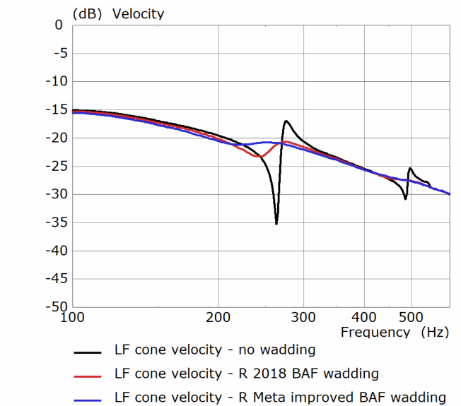
Figure 37. Measured LF cone velocity of R11 Meta showing the effect of standing waves and their improved damping
