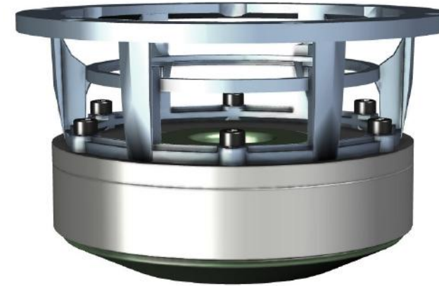
Figure 23. R Series (2018) Uni-Q rigid aluminium chassis directly affixed to motor
