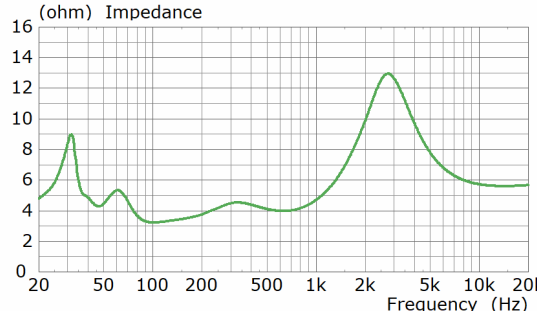
R5 Meta directivity contours - horizontal (top) and vertical (middle) - and impedance (bottom)
