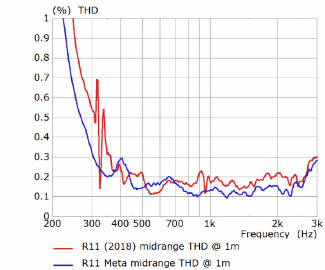
Figure 29. Comparison of measured THD (%) between R Series (2018) (red) and R Series with MAT (blue) as measured on an R11 enclosure without crossover at 90 dB SPL at 1m
