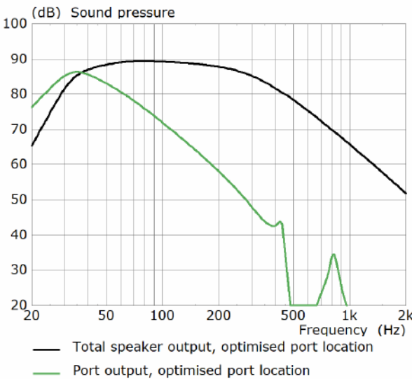
Figure 42. System output simulation showing the effect of optimised port location on standing wave leakage
