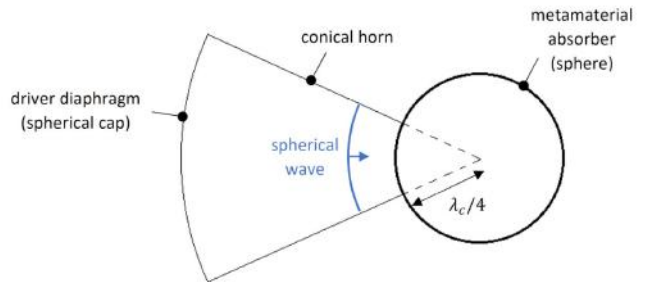
Figure 7. Geometric principle behind the coupling of the tweeter spherical dome to the metamaterial absorber
