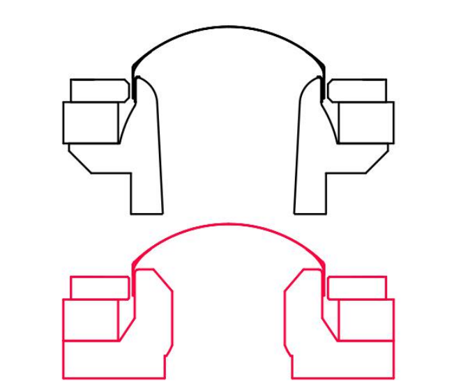
Figure 8. Comparison of tweeter motor geometries for R Series (2018) (red, bottom) and R Series with MAT (black, top)
