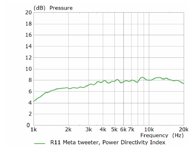
Figure 11. Tweeter Power Directivity Index (without crossover) as measured on R11 Meta
