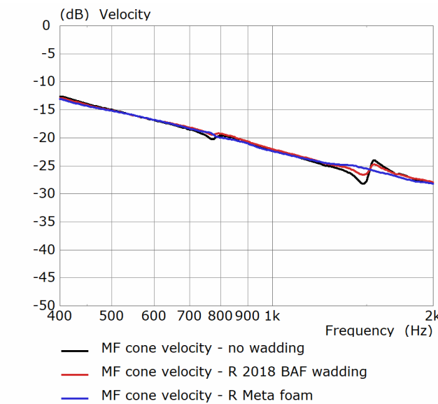
Figure 38. Measured midrange cone velocity of R11 Meta showing the effect of standing waves and their improved damping
