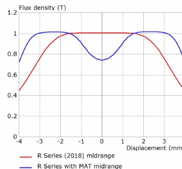
Figure 17. Midrange motor flux density B(x)
