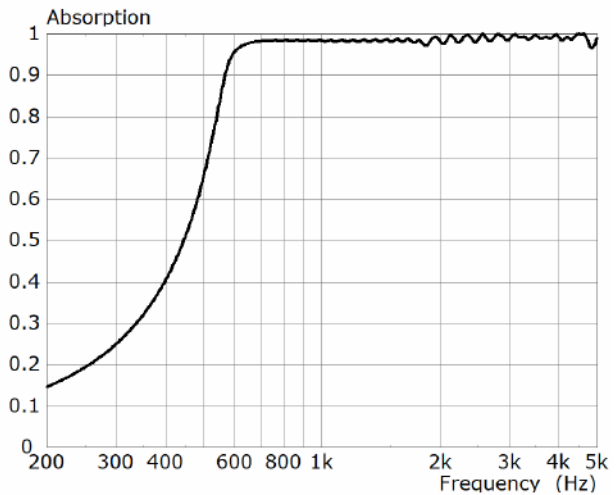
Figure 6. Absorption at the entrance of the conical duct, immediately behind the dome
