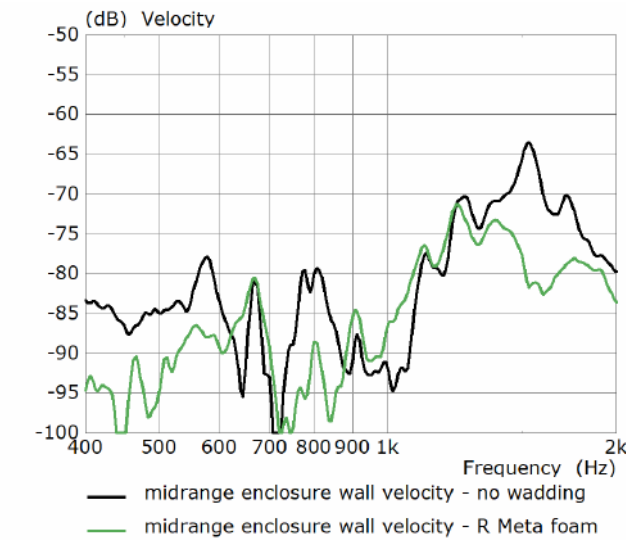
Figure 39. Measured surface velocity of cabinet wall outside midrange enclosure in R11 Meta comparing the standing wave leakage with and without acoustic damping
