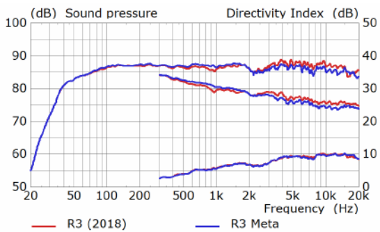
Figure 46. Axial frequency response, acoustic power average and acoustic power average directivity index of R3 (2018) (red) vs. R3 Meta (blue)
