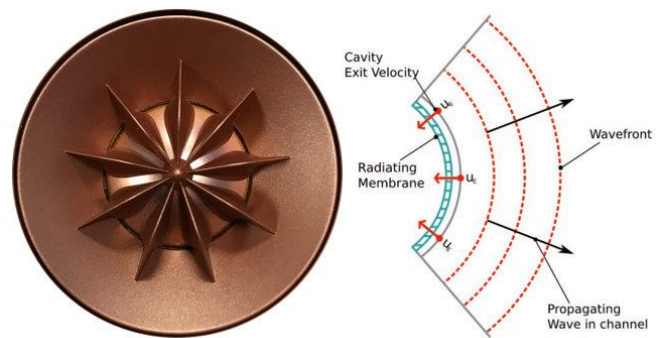
Figure 10. Tangerine Waveguide geometry
