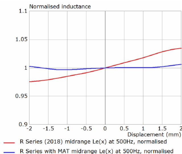
Figure 21. Comparison of normalised midrange voice coil inductance modulation with displacement at 500Hz
