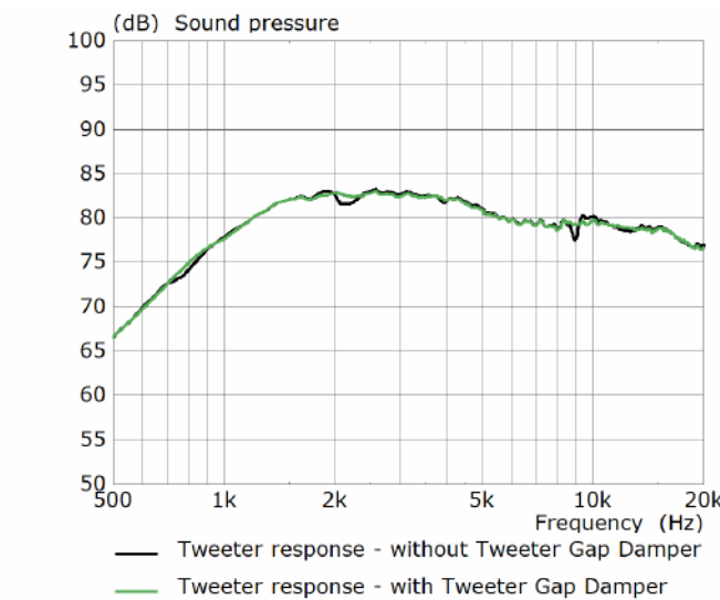
Figure 9. Improvement in tweeter frequency response due to the Tweeter Gap Damper
