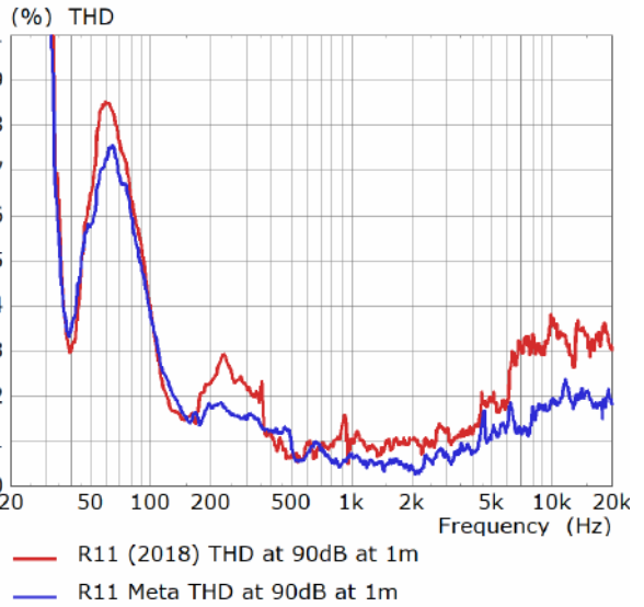
Figure 48. Comparison of THD (%) between R11 (2018) (red) and R11 Meta (blue) at 90dB SPL matched at 500Hz at 1m
