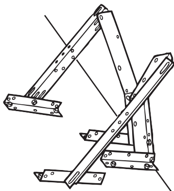
FIG. A, ROOF MOUNT
