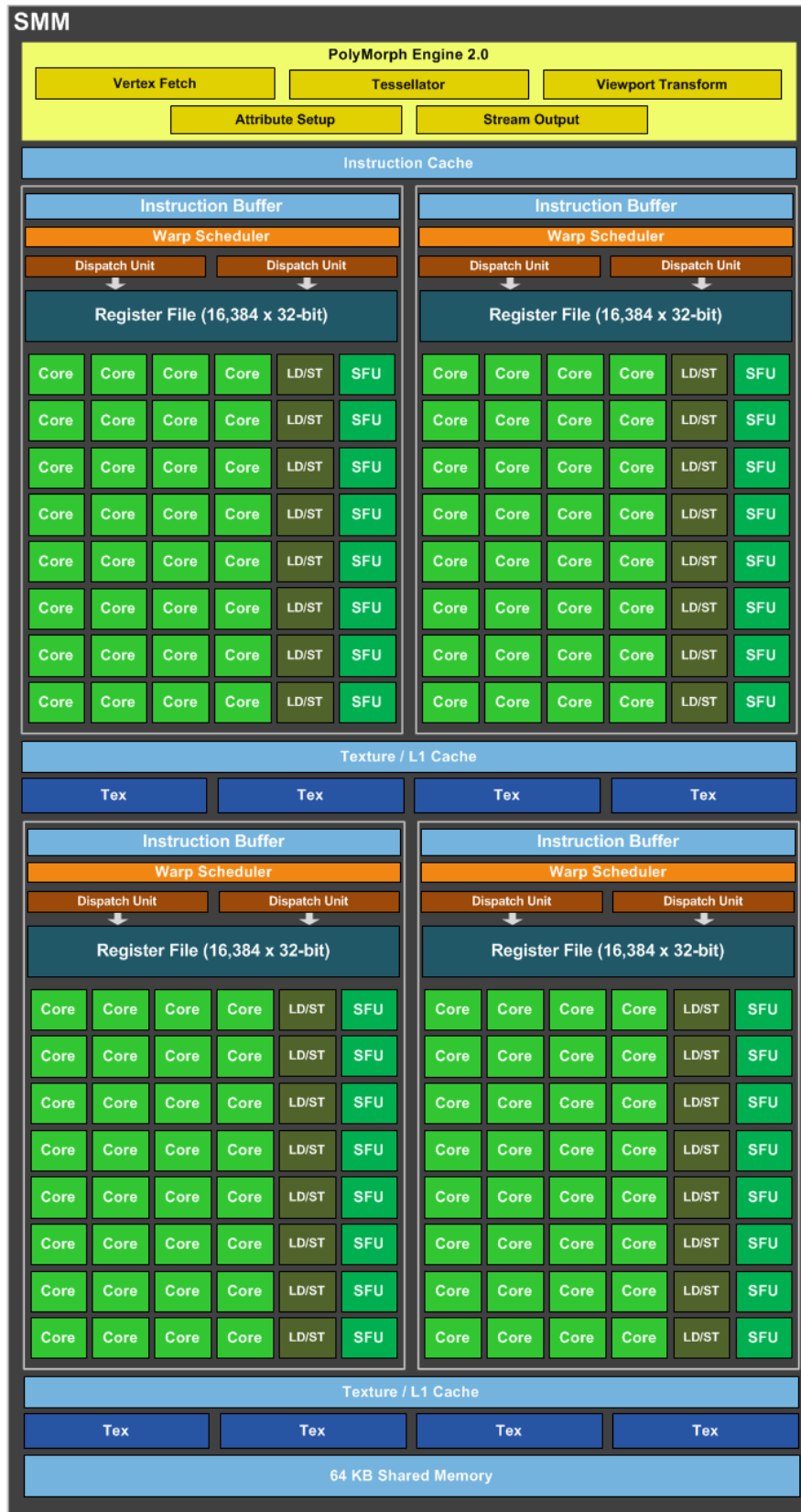
Figure 3: Maxwell SM Block Diagram
