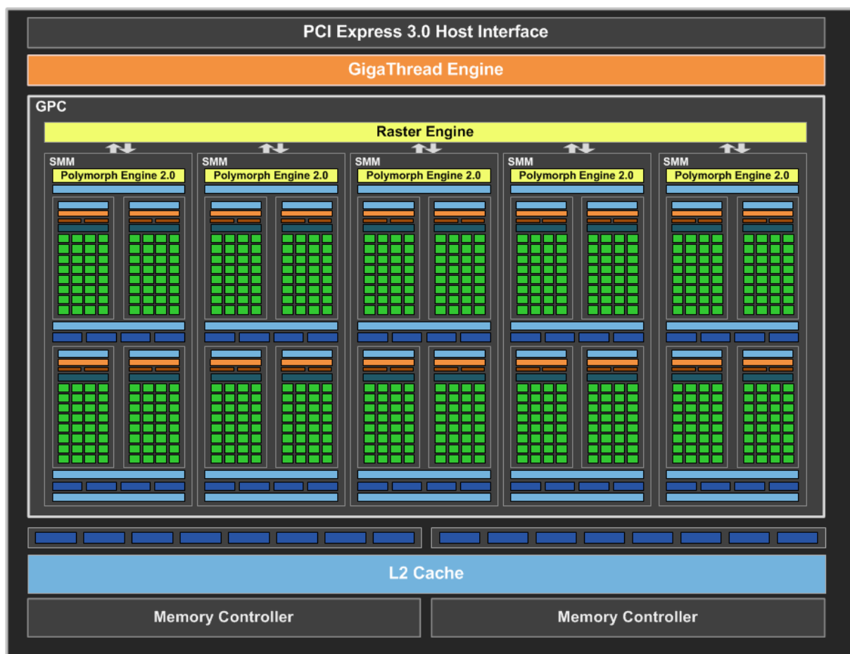
Figure 2: GM107 Full-Chip Block Diagram
